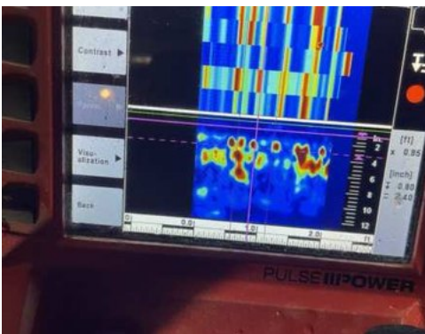
GPR scan display
